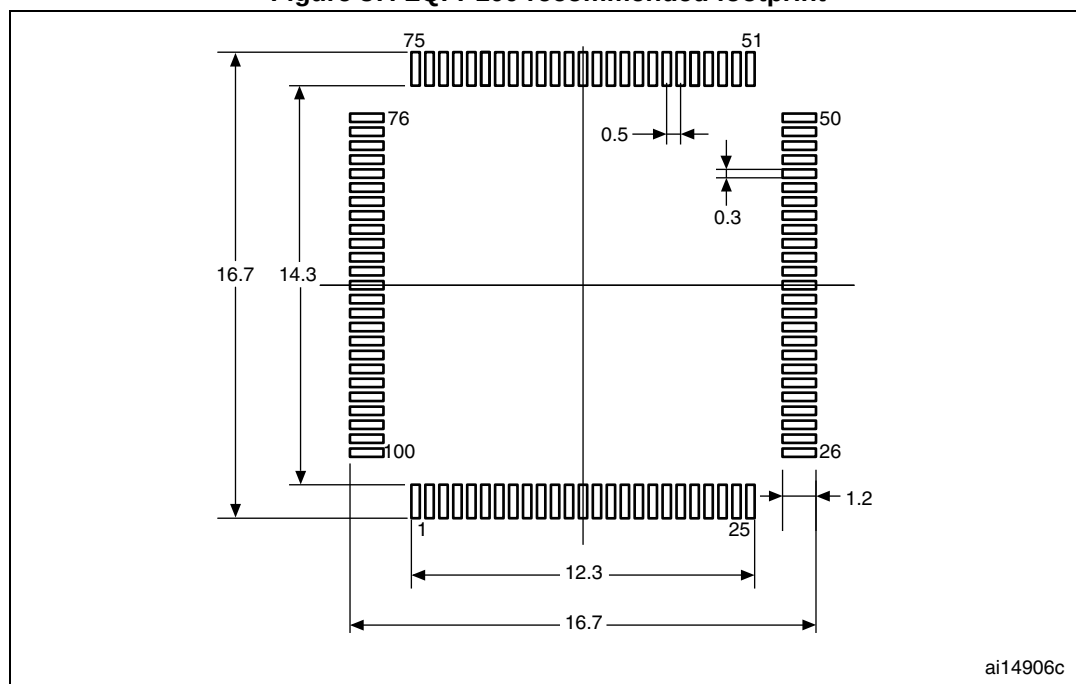
Figure 37. LQFP100 recommended footprint
