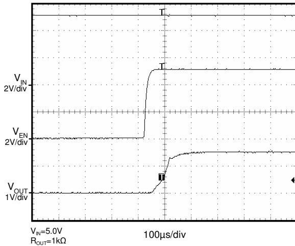
Start Up (Enable) ( V_{OUT}=1.5V )
