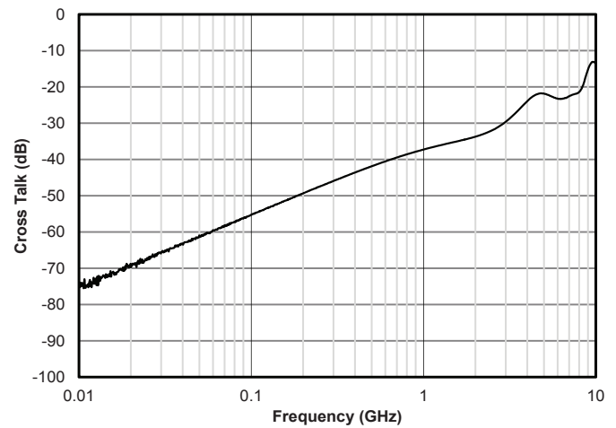
Analog Crosstalk
