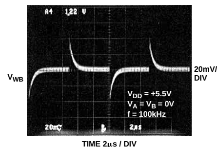
Figure 18. Digital Feedthrough
