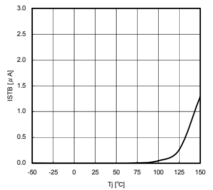
Fig.18 Tj-ICCSTB
