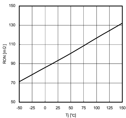
Fig.22 Tj-ROn ( V_{CC}=5\text{V}/V_o=1.2\text{V} )
