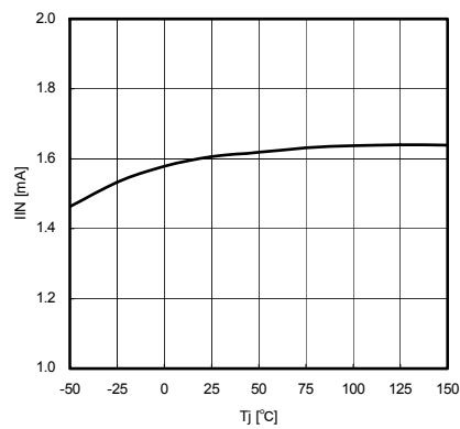
Fig.17 Tj-IIN
