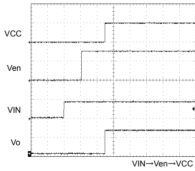
Fig.13 Input sequence
