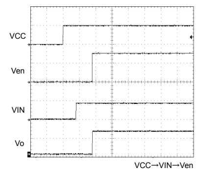
Fig.9 Input sequence
