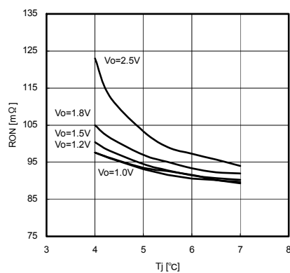
Fig.23 Vcc-ROn
