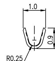
WIRE BARREL
