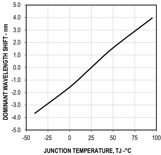
Figure 8: Wavelength vs. Temperature
