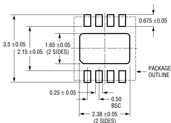
DD Package 8-Lead Plastic DFN (3mm × 3mm) (Reference LTC DWG # 05-08-1698)
