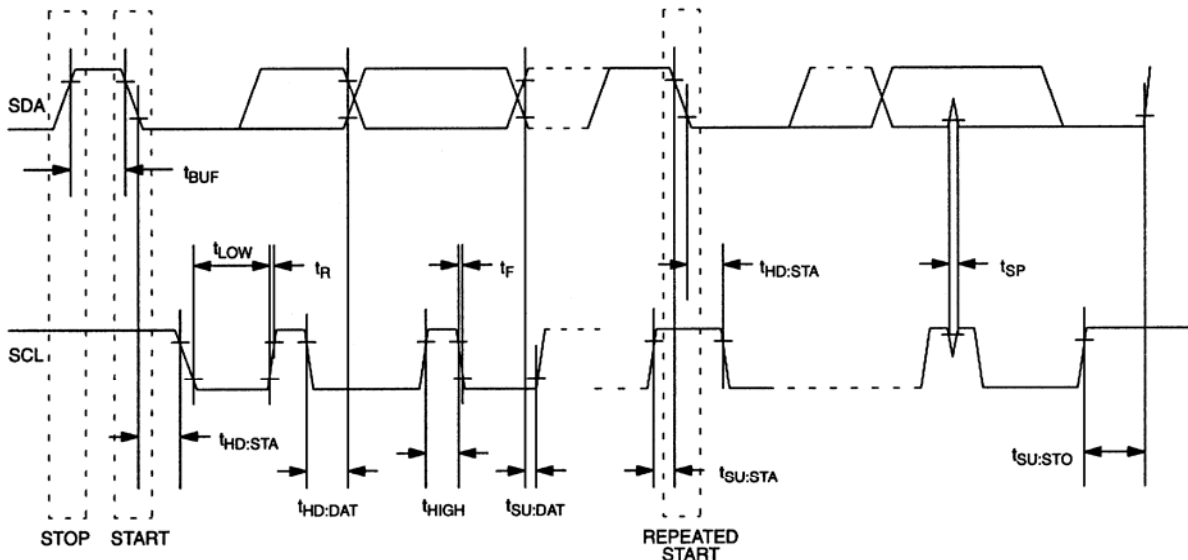
Figure 3. TIMING DIAGRAM
