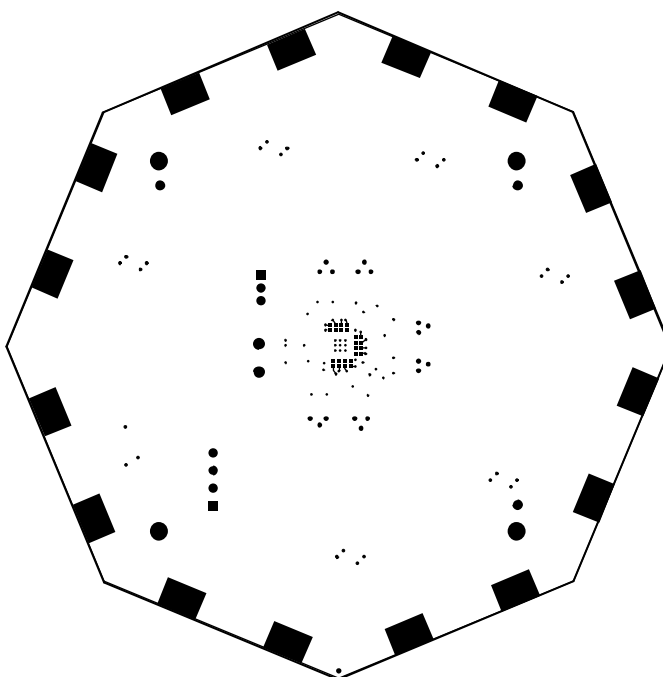
Figure 8. Bottom Trace Layer
