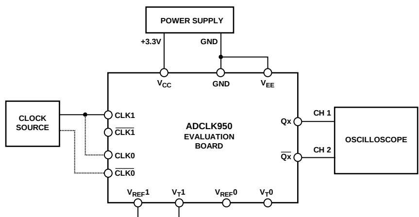
Figure 2. Recommended Setup for Device Evaluation
