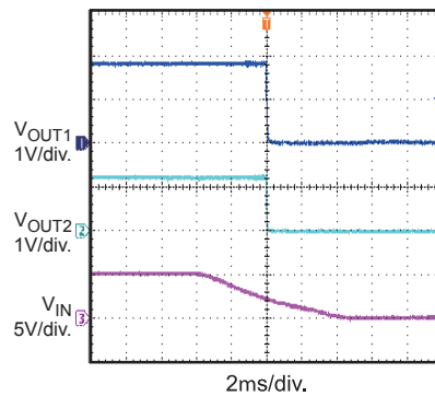
V in Power Down with Load
