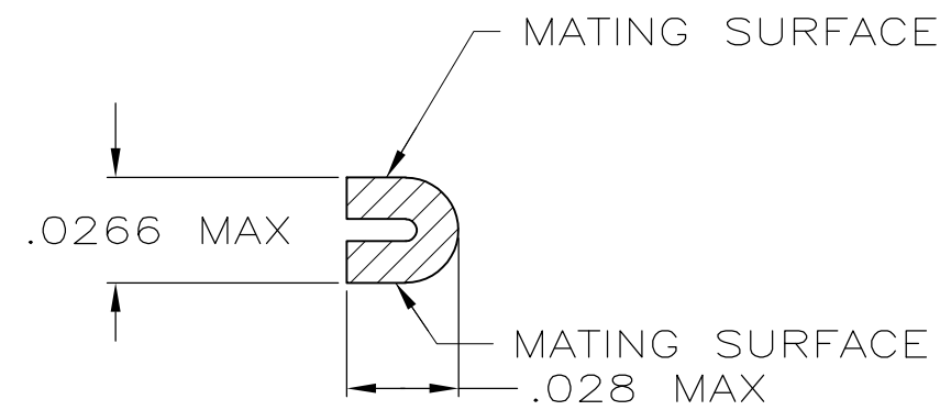
SECTION B-B
