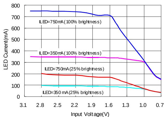
2. LED Current vs Input Voltage
