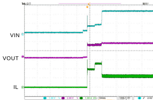
6. Start-Up Waveform
