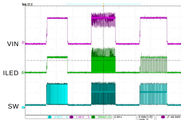
5. 3 Modes Change
