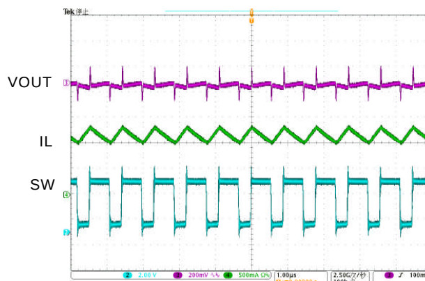
8. Switching Waveform
