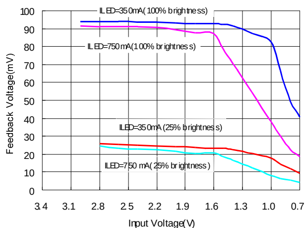
4. Feedback Voltage vs Input Voltage
