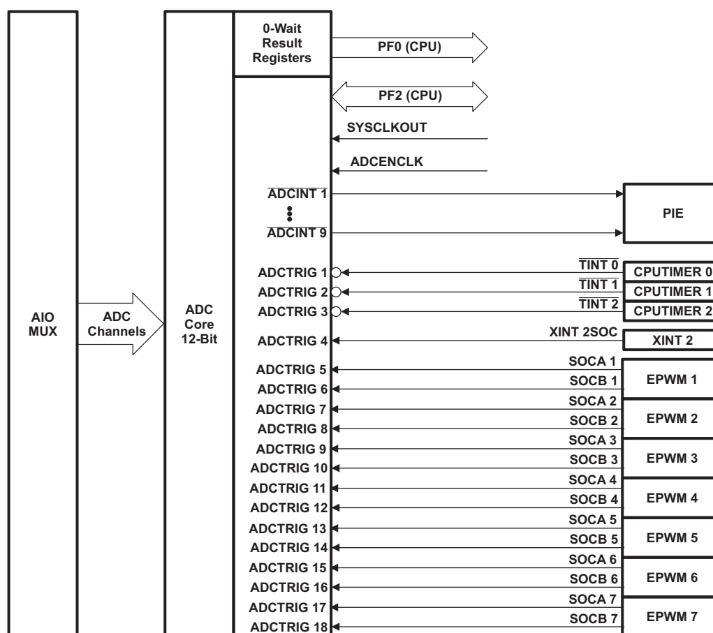
Figure 4-3. ADC Connections
