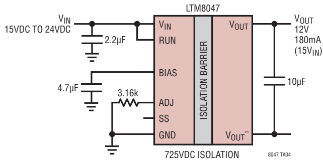
12V Isolated Flyback Converter
