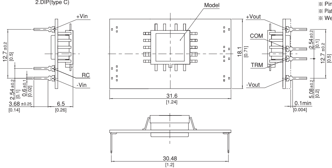
2.DIP(type C)
