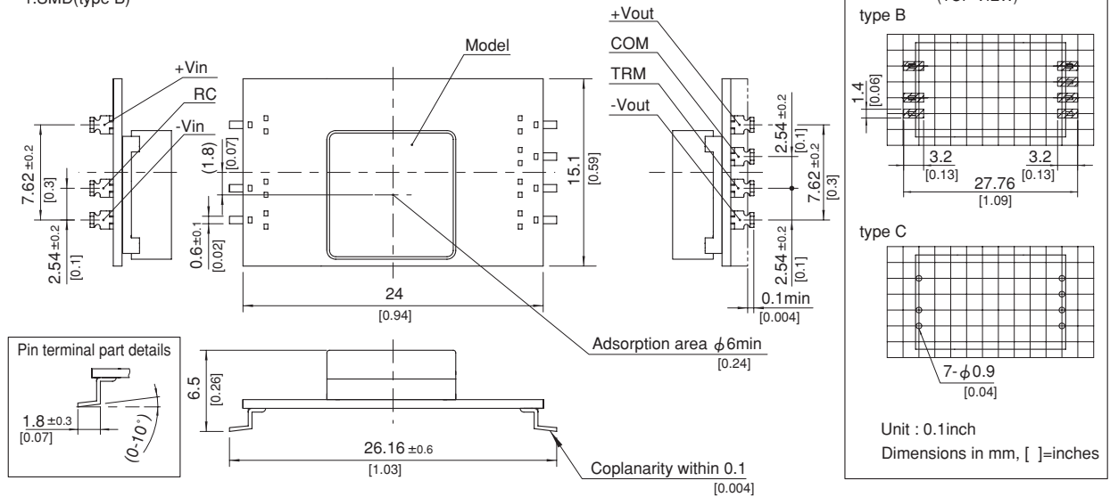
1.SMD(type B)
