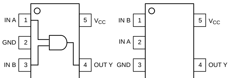
Figure 1. SOT-953 (Top Thru View)
