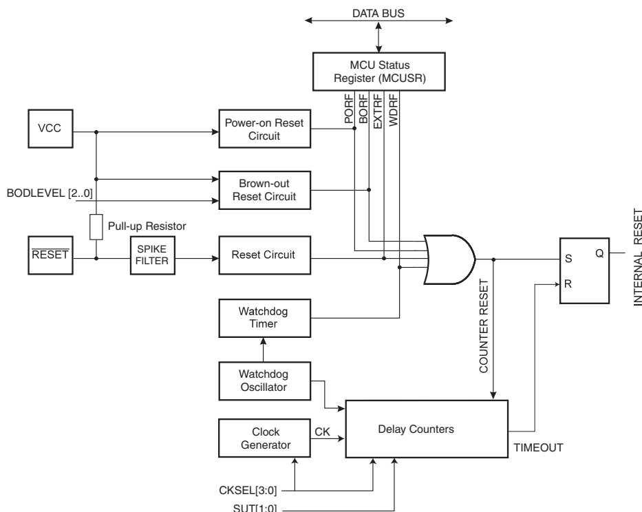
Figure 14. Reset Logic
