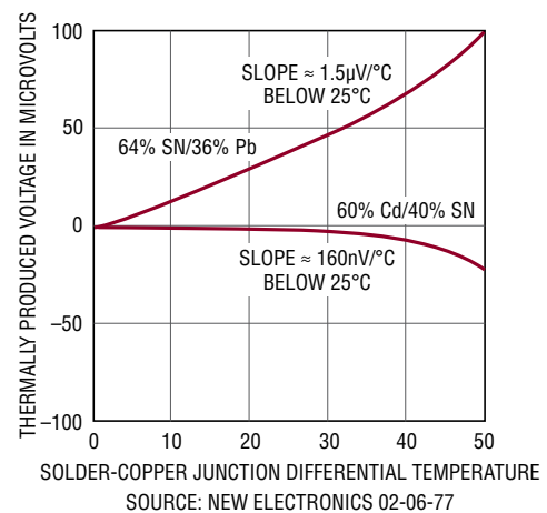
Figure 3. Solder-Copper Thermal EMFs
