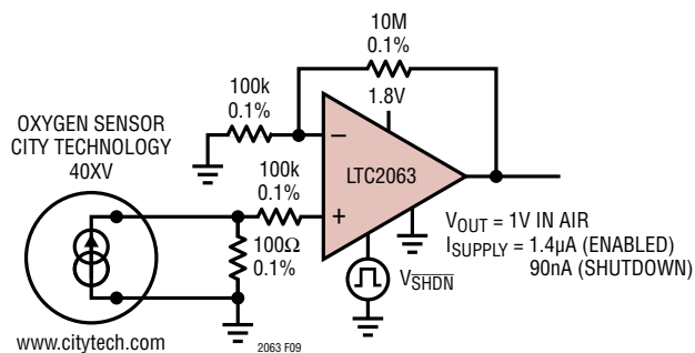
Figure 9. Micropower Precision Oxygen Sensor
