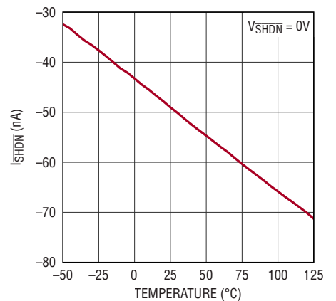
SHDN Pin Current vs Temperature
