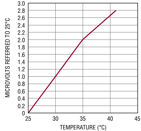
Figure 2. Thermal EMF Generated by Two Copper Wires from Different Manufacturers
