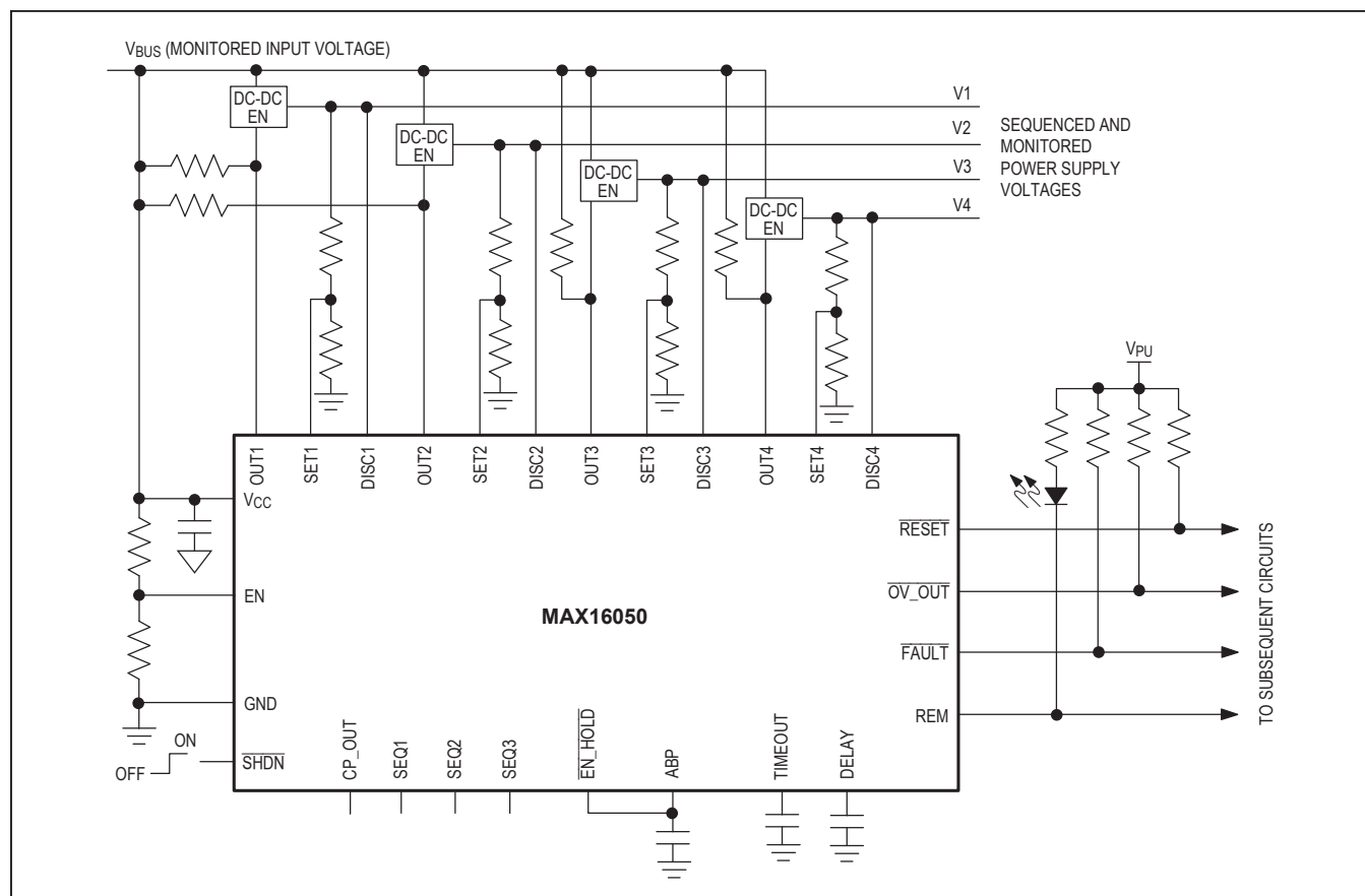
Figure 1. Typical Application Circuit for Sequencing Four DC-DC Converters
