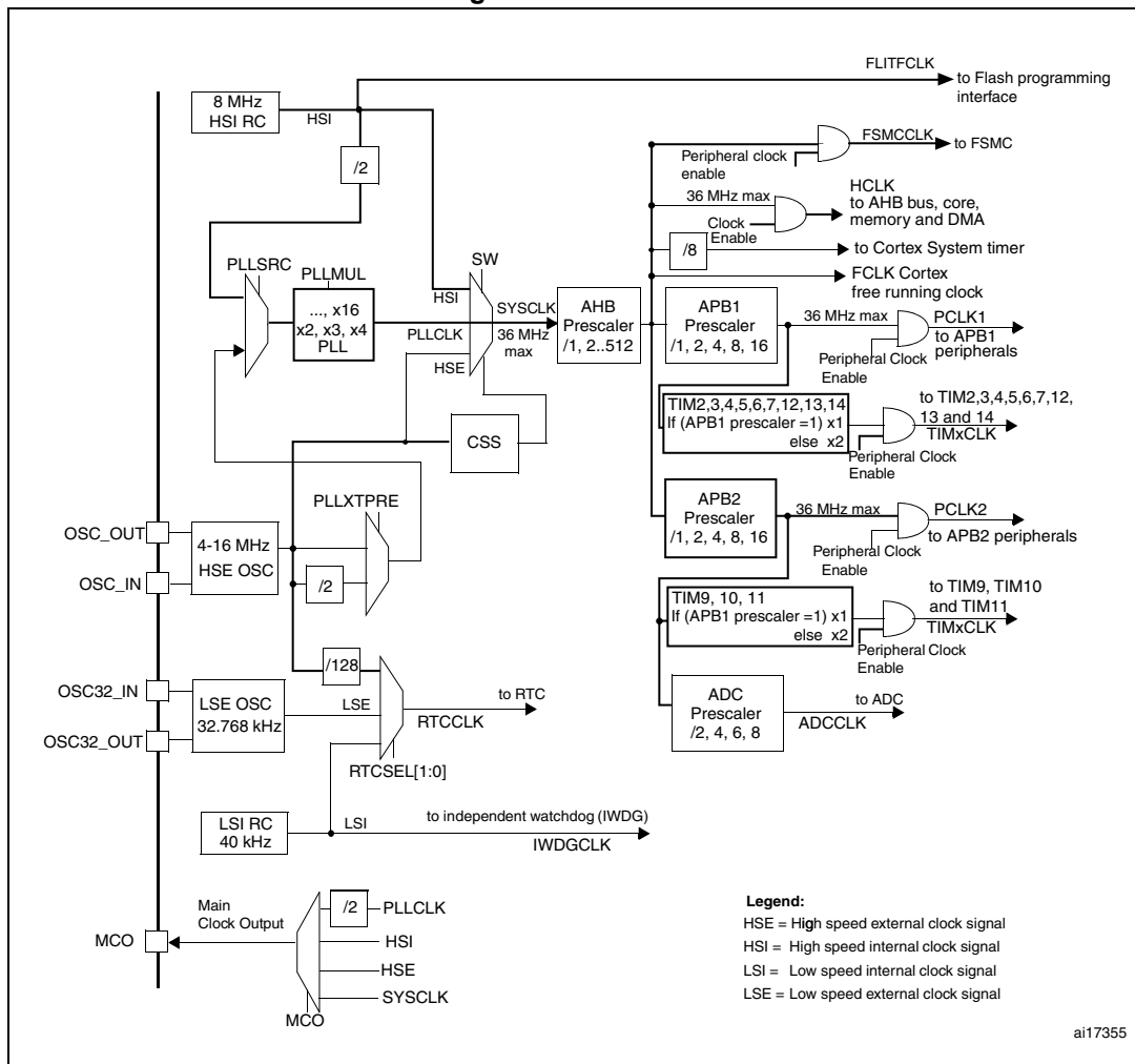
Figure 2. Clock tree
