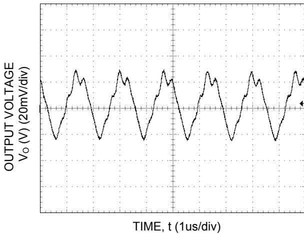
Fig-17. Typical output ripple and noise (CO=22 \mu F ceramic, VIN = 12V, I_o = I_{o,max} ).
