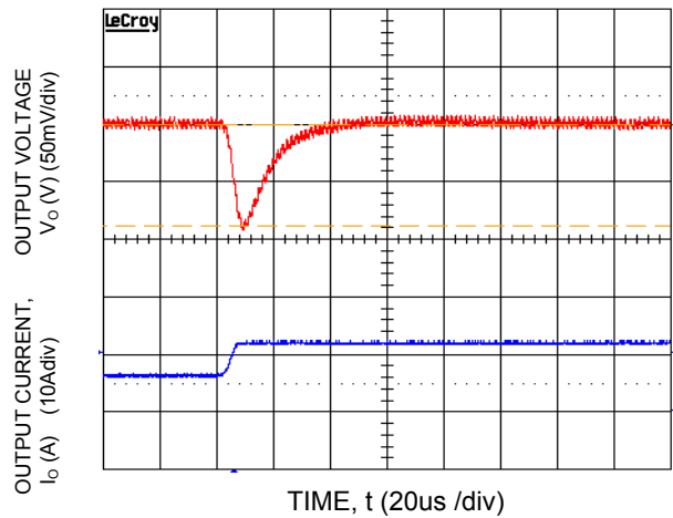
Fig-18. Transient Response to Dynamic Load Change from 50% to 100% at 12Vin, Cout= 5x47 \mu F, CTune=1500pF & RTune=330ohms
