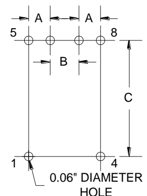
Board Layout
