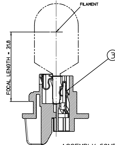
ASSEMBLY CONDITION
