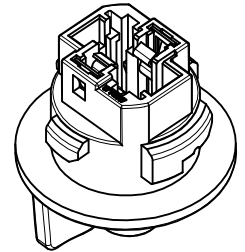
ISO VIEW
