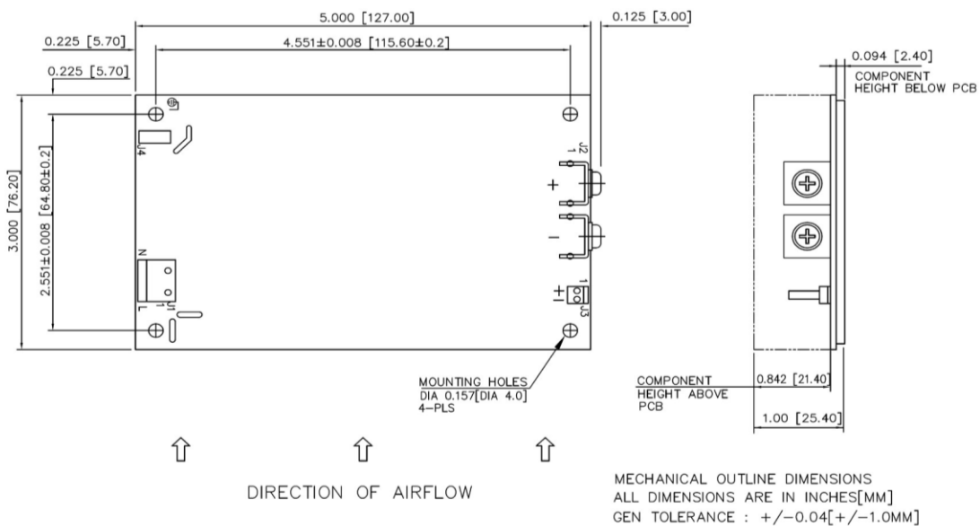
Figure 2. Mechanical Drawing - Screw Terminal (Option 1)
