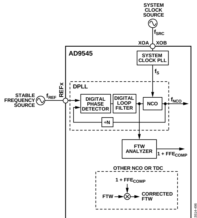
Figure 104. Closed-Loop Method
