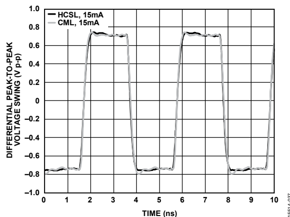
Figure 18. 245.76 MHz Output Waveform for 15 mA Driver Settings; HCSL Drivers Terminated 50\ \Omega to GND per Figure 38; CML Drivers Terminated 50\ \Omega to 1.8 V per Figure 39
