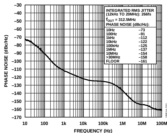
Figure 13. Absolute Phase Noise (PLL1, Configuration 5, HCSL Mode, f_{REF} = 25\text{ MHz} , f_{OUT} = 312.5\text{ MHz} , f_{OSC} = 52\text{ MHz} Crystal, 50 Hz DPLL BW, Phase Buildout Mode)
