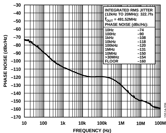
Figure 11. Absolute Phase Noise (PLL1, Configuration 3, HCSL Mode, f_{REF} = 1\text{ Hz} , f_{OUT} = 491.52\text{ MHz} , f_{COMP} = 19.2\text{ MHz} TCXO, f_{OSC} = 52\text{ MHz} Crystal, 0.5 Hz DPLL BW)
