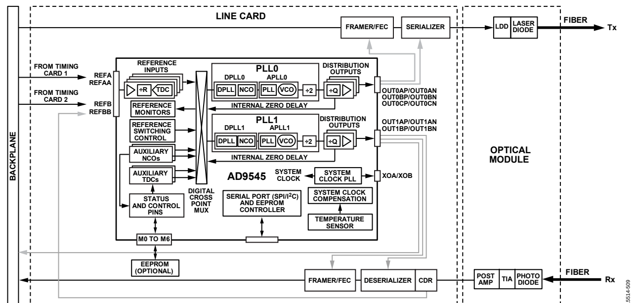
Figure 117. Optical Line Card Loop Timing Example
