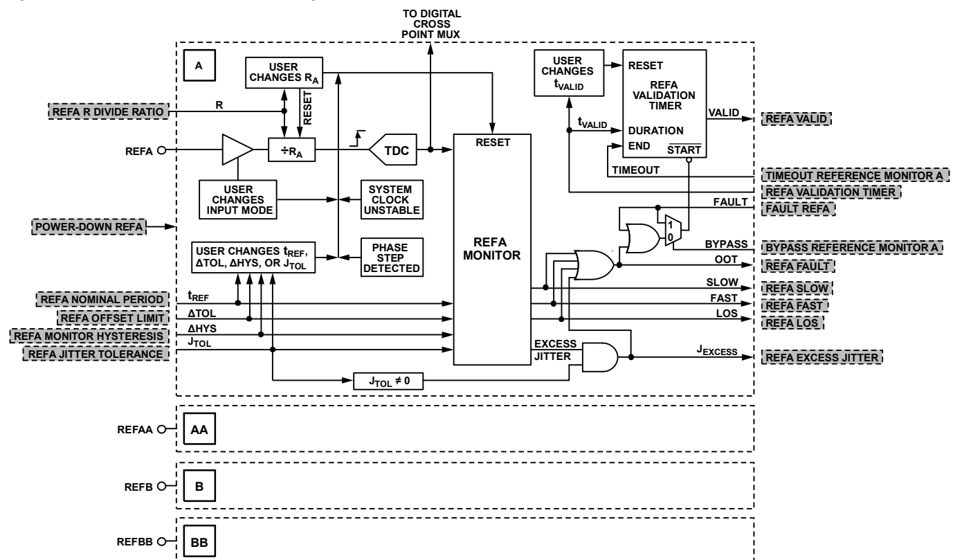
Figure 49. Reference Monitor
