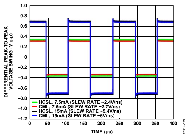
Figure 16. 8 kHz Output Waveforms for Various Driver Settings; HCSL Drivers Terminated 50\ \Omega to GND per Figure 38; CML Drivers Terminated 50\ \Omega to 1.8 V per Figure 39
