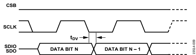
Figure 126. Timing Diagram for Serial Control Port Register Read—MSB First
