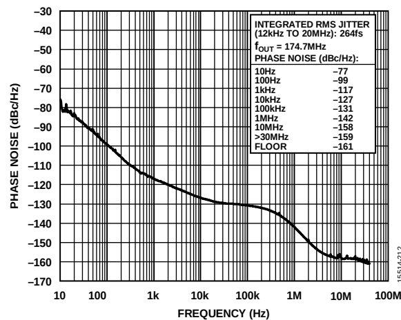
Figure 14. Absolute Phase Noise (PLL1, Configuration 6, HCSL Mode, f_{REF} = 155.52\text{ MHz} , f_{OUT} = 174.7\text{ MHz} , f_{OSC} = 52\text{ MHz} Crystal, 50 Hz DPLL BW, Phase Buildout Mode)
