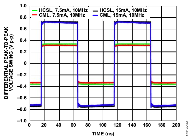
Figure 17. 10 MHz Output Waveforms for Various Driver Settings; HCSL Drivers Terminated 50\ \Omega to GND per Figure 38; CML Drivers Terminated 50\ \Omega to 1.8 V per Figure 39
