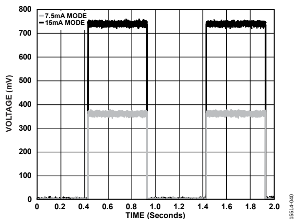
Figure 15. DC-Coupled, Single-Ended, 1 Hz Output Waveforms Using HCSL 7.5 mA and 15 mA Mode Terminated 50\ \Omega to GND per Figure 45; Slew Rate: \sim 7\text{ V/ns} for 15 mA Mode; \sim 3.5\text{ V/ns} for 7.5 mA Mode
