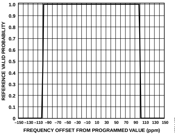
Figure 28. Reference Monitor Reference Valid Probability vs. Reference Input Frequency Offset; Tolerance = 100 ppm; Hysteresis = 0
