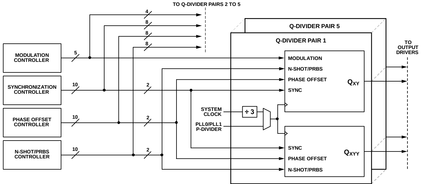
Figure 53. Functional Block Diagram of Q-Dividers and Controllers
