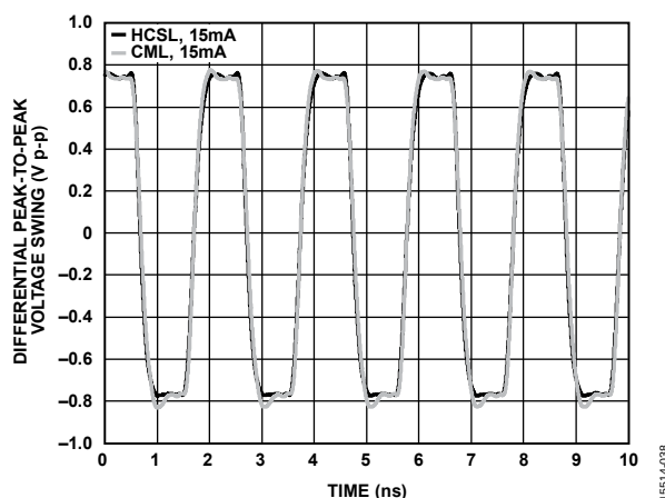
Figure 19. 491.52 MHz Output Waveform for 15 mA Driver Settings; HCSL Drivers Terminated 50\ \Omega to GND per Figure 38; CML Drivers Terminated 50\ \Omega to 1.8 V per Figure 39
