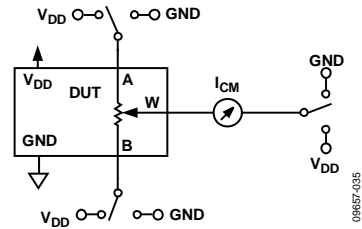
Figure 37. Common-Mode Leakage Current
