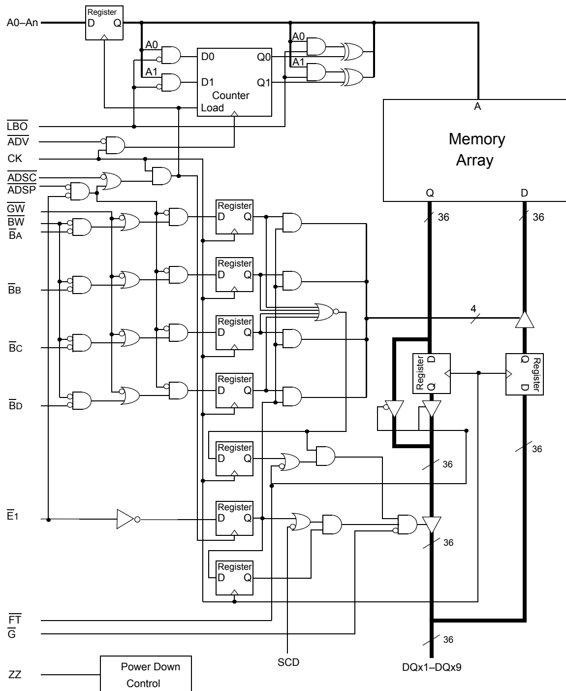
GS832218/36A Block Diagram
