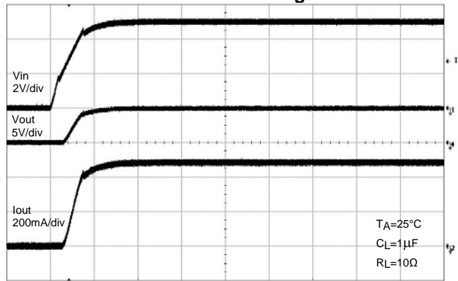
UVLO Increasing
