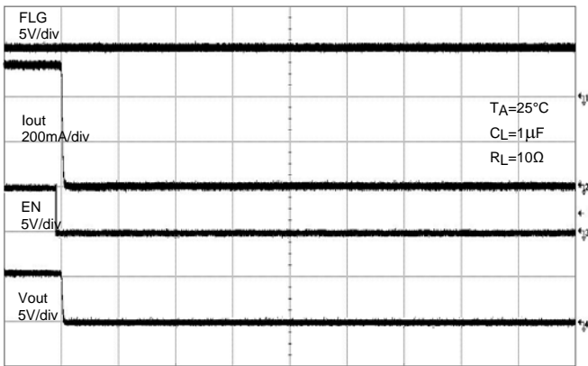
Device Disabled
