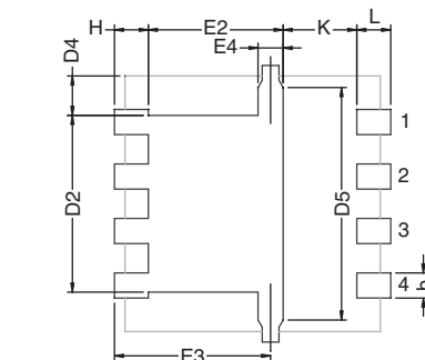
Backside View of Single Pad
