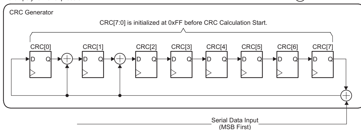
Figure 3-4. CRC Generator 8-bit Polynomial Expression
