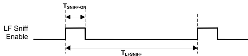
Figure 3-15. LF Sniffing Timing
