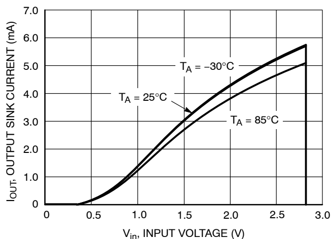
Figure 18. NCP304H/5L Series 2.7 V Reset Output Sink Current vs. Input Voltage
