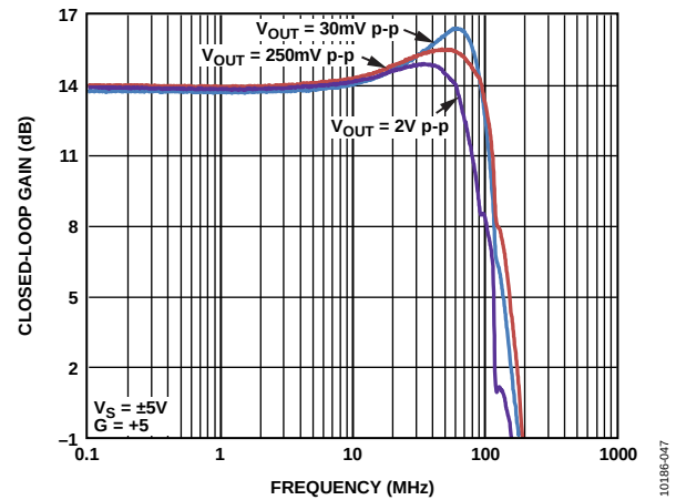
Figure 44. Frequency Response for G = +5
