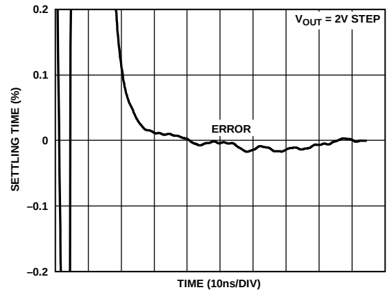
Figure 26. Settling Time to 0.1%
