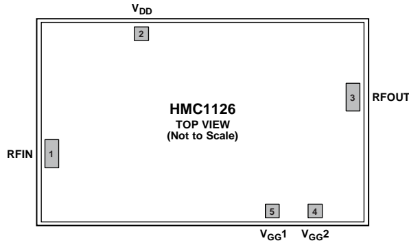
Figure 2. Pad Configuration
