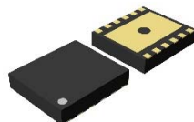
DFN(PLP)2730-12 2.70 x 3.00 x 0.6 (1) mm ( 1 ) maximum dimension
