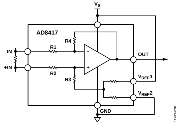
Figure 30. Split Supply
