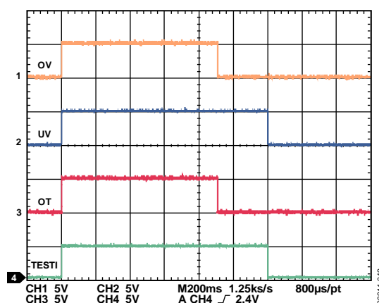
Figure 37. TESTI and AVOUTxx, Deglitch Time = 0.1 sec, Self-Test Fails (UV)
