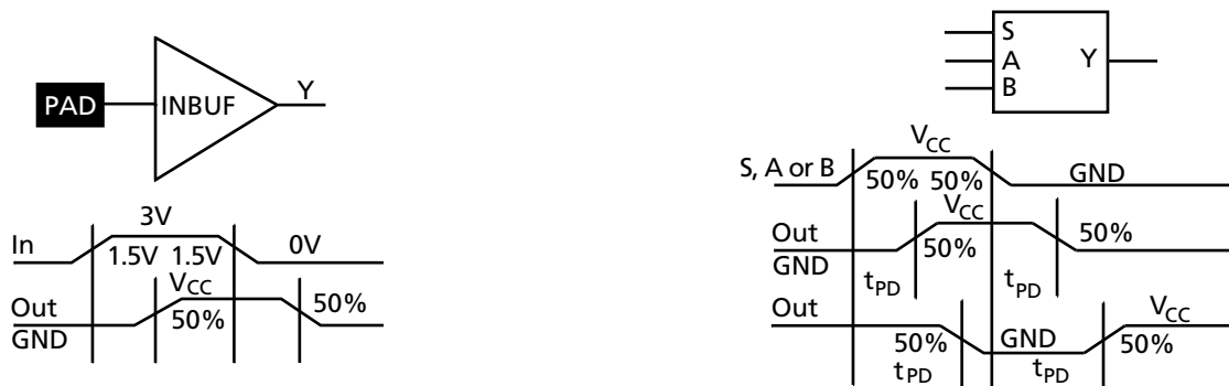
Figure 1-16 • Input Buffer Delays
