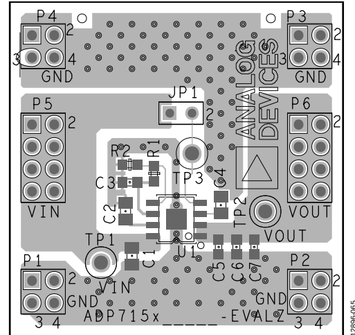
Figure 63. Sample 8-Lead SOIC PCB Layout
