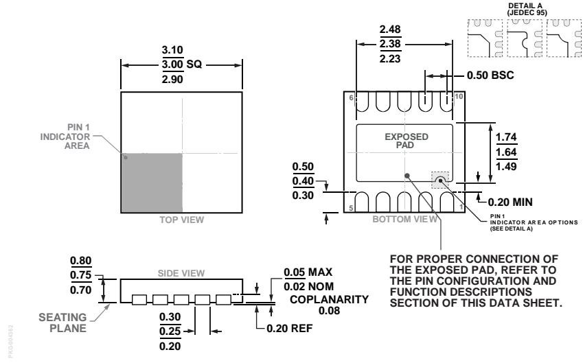
Figure 64. 10-Lead Lead Frame Chip Scale Package [LFCSP] 3 mm × 3 mm Body and 0.75 mm Package Height (CP-10-9) Dimensions shown in millimeters
