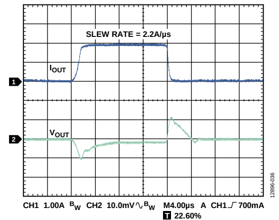
Figure 34. Load Transient Response, I_{\text{LOAD}} = 100\text{mA} to 2\text{A} , V_{\text{OUT}} = 3.3\text{V} , V_{\text{IN}} = 4.0\text{V} , C_{\text{OUT}} = 22\mu\text{F} , Channel 1 = I_{\text{OUT}} , Channel 2 = V_{\text{OUT}}
