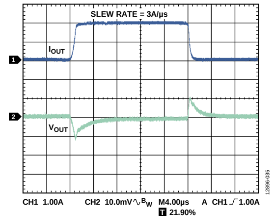
Figure 33. Load Transient Response, I_{\text{LOAD}} = 100\text{mA} to 2\text{A} , V_{\text{OUT}} = 3.3\text{V} , V_{\text{IN}} = 4.0\text{V} , Channel 1 = I_{\text{OUT}} , Channel 2 = V_{\text{OUT}}
