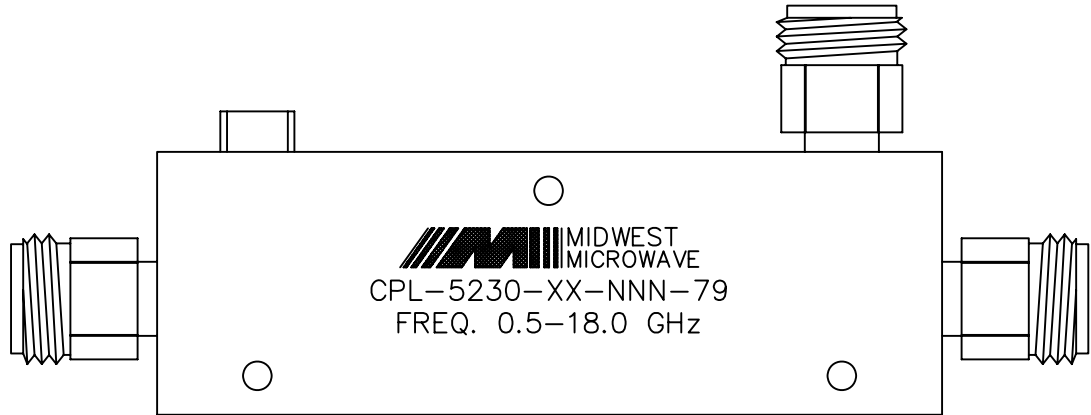
BACKSIDE MARKING
