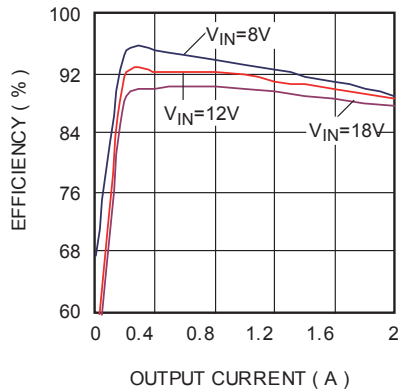
Efficiency vs. Load Current V OUT =5V
