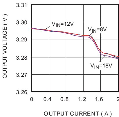
Load Regulation V OUT =3.3V
