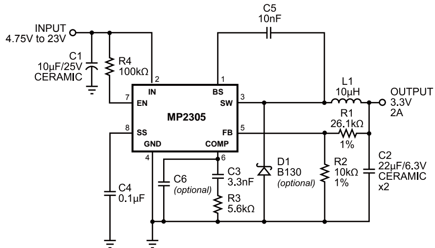
Figure 3—MP2305 with 3.3V Output, 22 \mu F/6.3V Ceramic Output Capacitor
