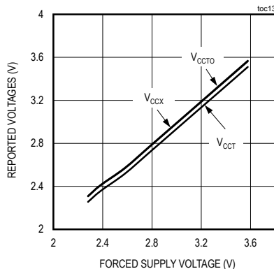
REPORTED V CCTO , V CCX , V CCT VOLTAGES vs. FORCED SUPPLY VOLTAGE
