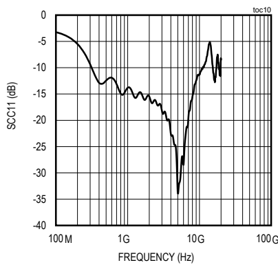
Tx INPUT COMMON-MODE RETURN LOSS vs. FREQUENCY
