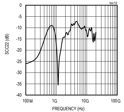
Tx OUTPUT COMMON-MODE RETURN LOSS vs. FREQUENCY
