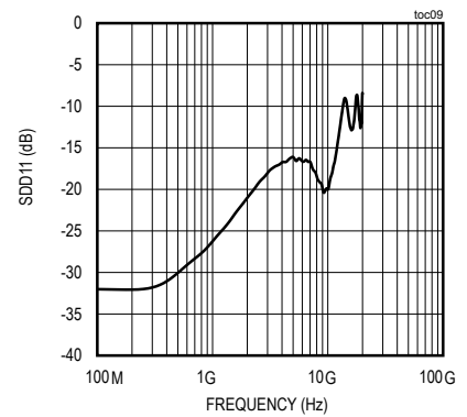
Tx INPUT DIFFERENTIAL RETURN LOSS vs. FREQUENCY
