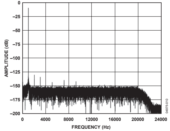
Figure 9. Low Power FFT, 1 kHz, -6\text{ dB} Input Tone, 256x Decimation
