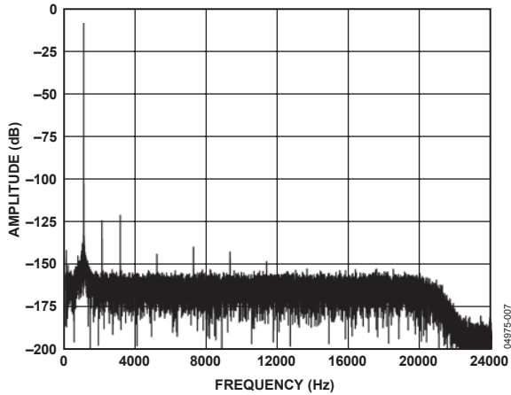
Figure 6. Normal Mode FFT, 1 kHz, -6\text{ dB} Input Tone, 256x Decimation
