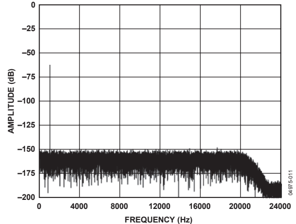
Figure 10. Low Power FFT, 1 kHz, -60\text{ dB} Input Tone, 256x Decimation
