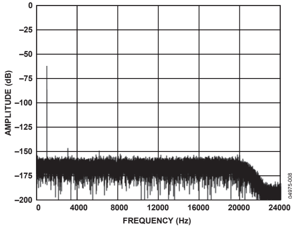
Figure 7. Normal Mode FFT, 1 kHz, -60\text{ dB} Input Tone, 256x Decimation
