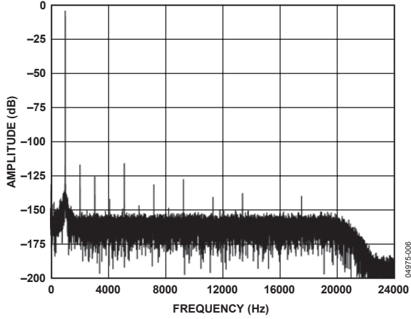
Figure 5. Normal Mode FFT, 1 kHz, -0.5\text{ dB} Input Tone, 256x Decimation
