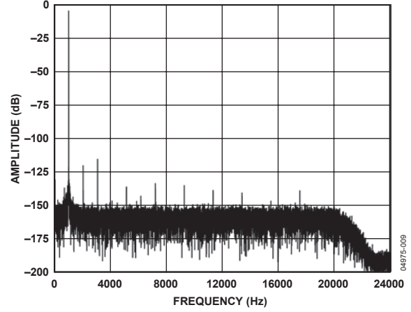
Figure 8. Low Power FFT, 1 kHz, -0.5\text{ dB} Input Tone, 256x Decimation
