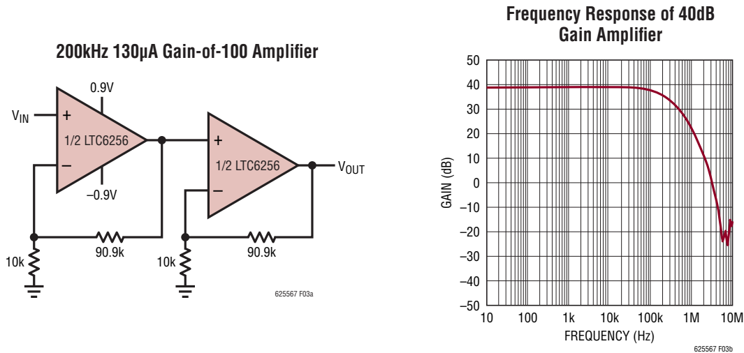
Figure 3. Gain of 100 Amplifier (3dB Bandwidth of 200kHz on 130 \mu A Supply Current)
